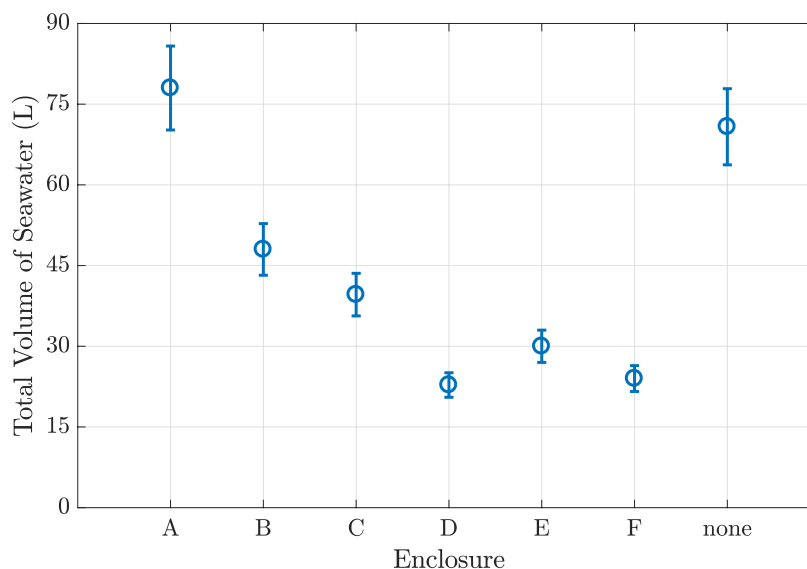
Figure 6: Total volume of seawater to come in contact with \text{MnO}_2 impregnated acrylic fibers in different enclosure types as determined by ^{226}\text{Ra} count using \gamma -spectrometry.
