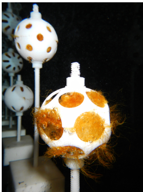
Figure 5: Shell enclosures in the recirculating flume, each containing a small, pre-weighed, mass of adsorbent fiber. Samples were taken by snipping small pieces ( \sim 35 mg) using Teflon coated scissors from sections of the adsorbent fiber in each enclosure and from the control.
