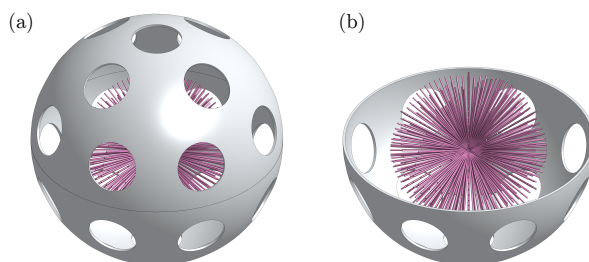
53 Figure 1: Initial adsorbent concept with decoupling of mechanical and chemical requirements. 54 Soft, inner adsorbent sphere is encased in tough, outer protective sphere. Outer sphere 55 features holes to allow adequate seawater to adsorbent interior. [13]
