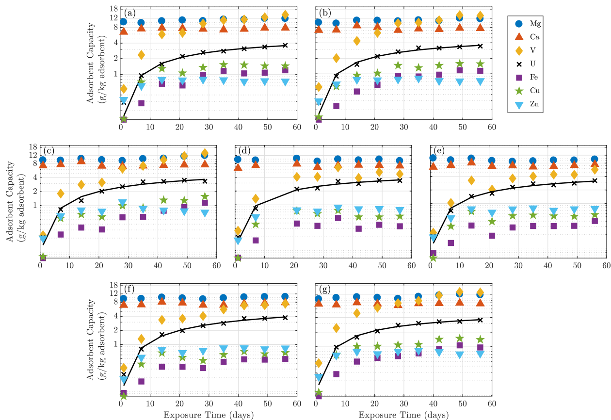
Figure 7: Time-dependent measurements of adsorption capacities (g element/kg adsorbent) for several trace elements retained by the ORNL AI8 adsorbent exposed to filtered natural seawater in a flume in various shell enclosures, (a)-(f) (as shown in figure 3), and without any enclosure, (g). The black line drawn through the uranium adsorption data represents fitting to a one-site ligand model (equation 4)
